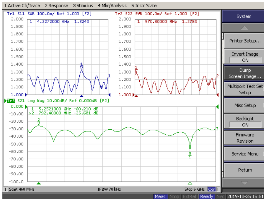
TR1: P2 Port VSWR, TR2: P3 Port VSWR, TR3: P2-P3 Isolation
