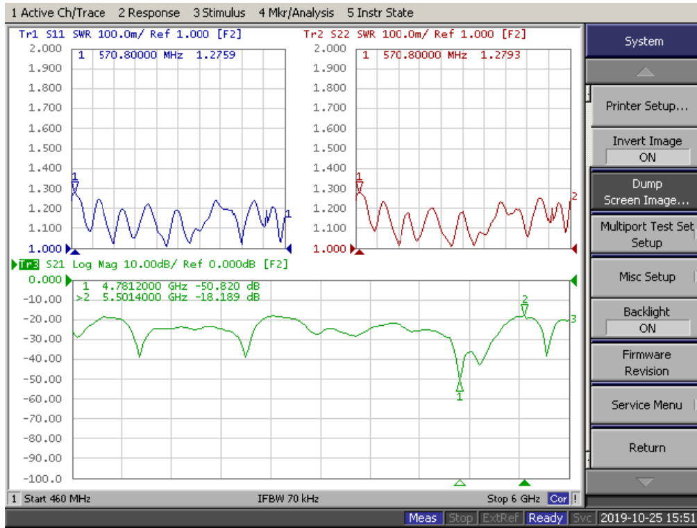
TR1: P1 Port VSWR, TR2: P2 Port VSWR, TR3: P1-P2 Isolation
