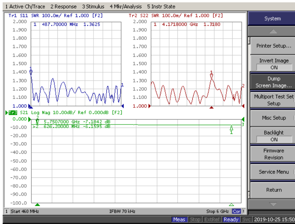
TR1: SUM Port VSWR, TR2: P3 Port VSWR, TR3: SUM-P3 Port Insertion Loss
