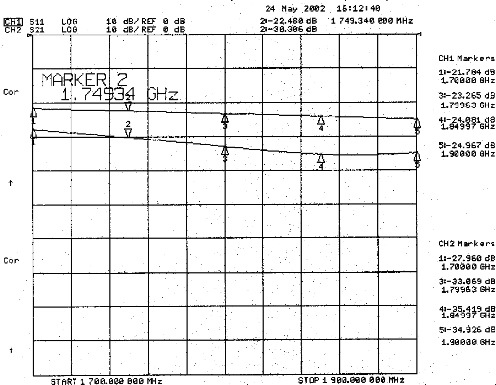
TR1: P2 PORT RETURN LOSS, TR2: ISOLATION (P2-P3)
