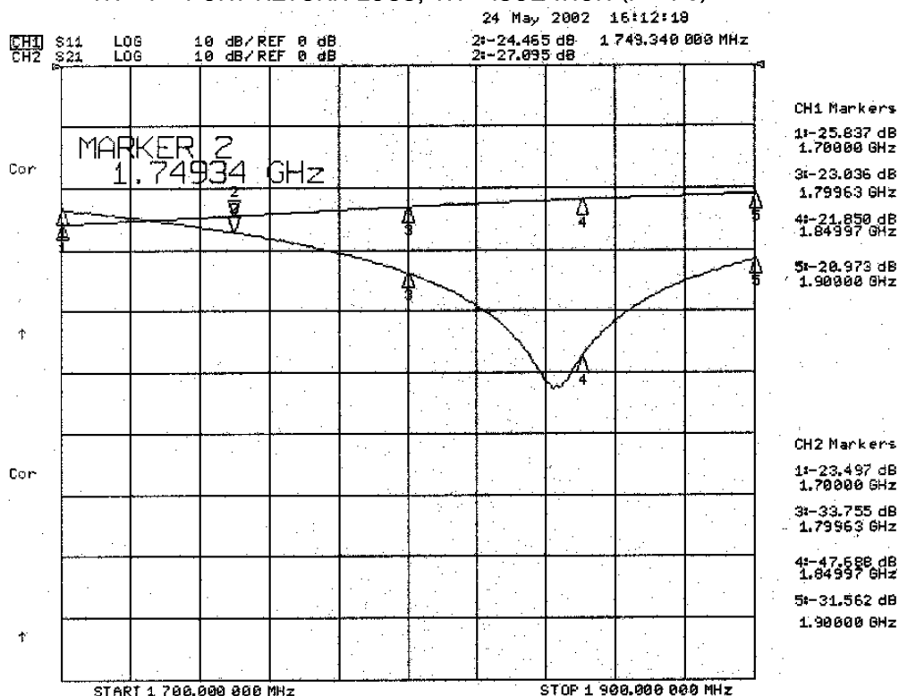
TR1: P1 PORT RETURN LOSS, TR2: ISOLATION (P1-P3)
