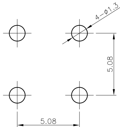
PCB MOUNTING HOLE SIZE (SCALE 5:1)
