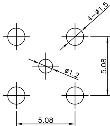
PCB MOUNTING HOLE SIZE
