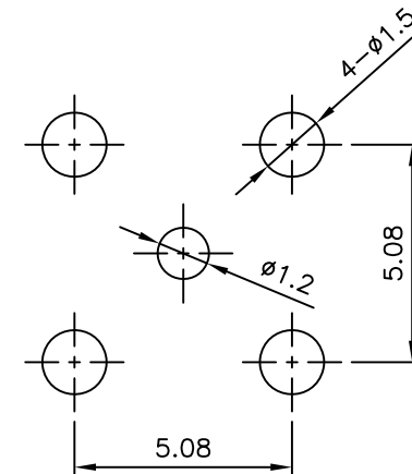
PCB MOUNTING HOLE SIZE
