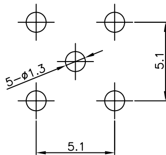
PCB MOUNTING HOLE DIMENSION (4:1)
