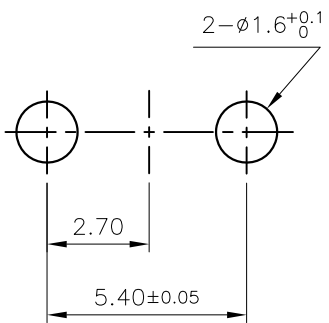
PCB MOUNTING HOLE
