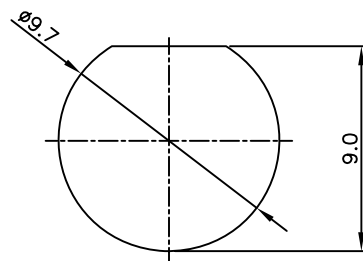
PANEL MOUNTING HOLE SIZE
