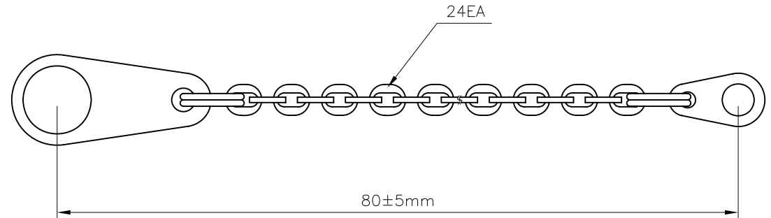
CHAIN DETAIL
