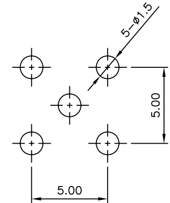
PCB MOUNTING HOLE SIZE
