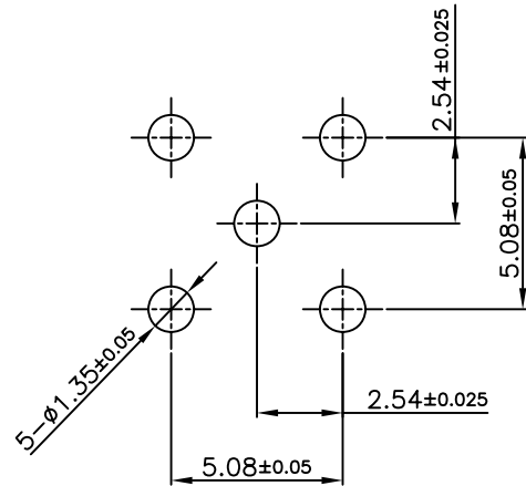
PCB MOUNTING HOLE DIMENSION (4:1)
