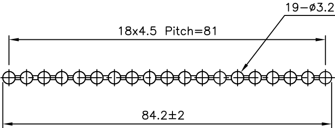
ROUND WIRE DETAIL (SCALE 1:1)
