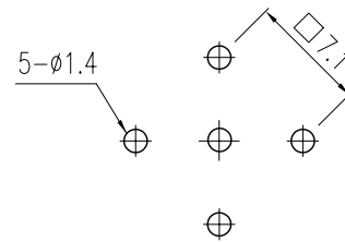
PCB MOUNTING HOLE
