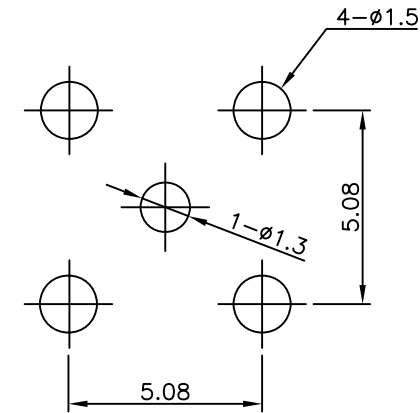
PCB MOUNTING HOLE SIZE
