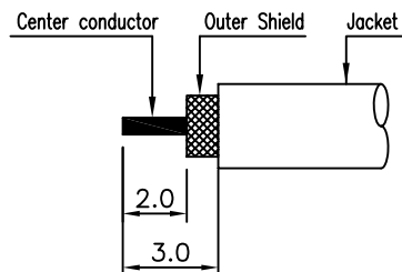
141F CABLE STRIP
