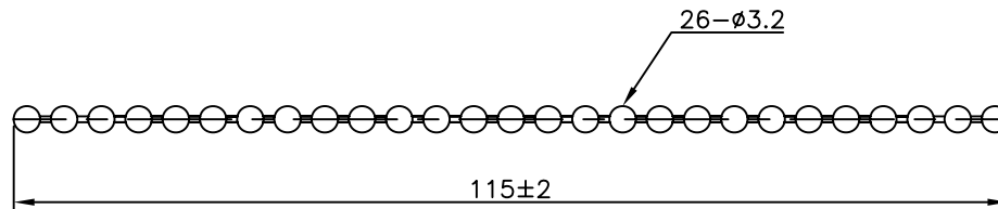
ROUND WIRE DETAIL (SCALE 1:1)
