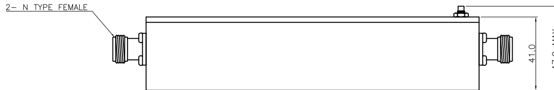
SIDE VIEW
