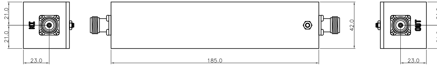
TOP VIEW
