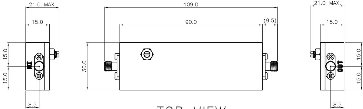
TOP VIEW
