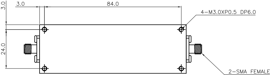
BOTTOM VIEW
