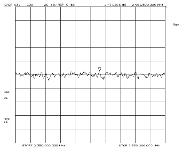
# Rejection[2.35~2.55GHz]
