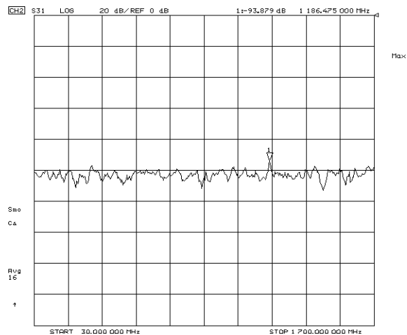
# Rejection[DC~1700MHz]
