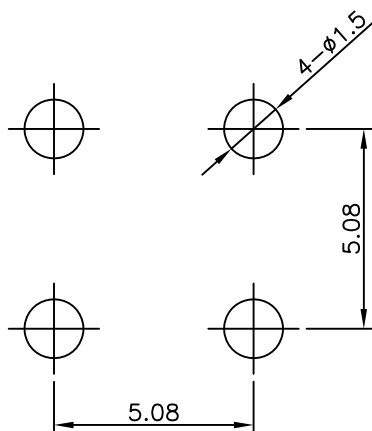
PCB MOUNTING HOLE SIZE (SCALE 5:1)
