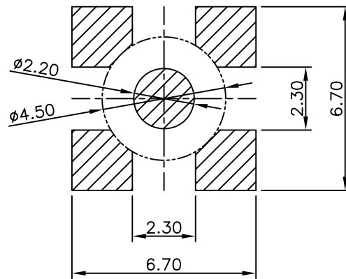
PCB LAYOUT (SCALE 5:1)
