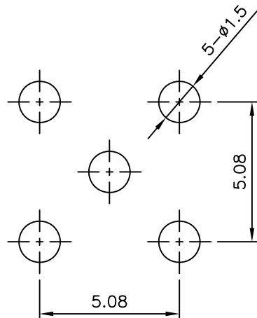
PCB MOUNTING HOLE SIZE
