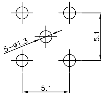
PCB MOUNTING HOLE DIMENSION (4:1)
