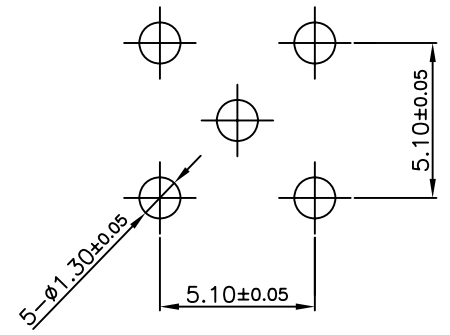
PCB MOUNTING HOLE SIZE
