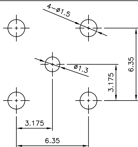
PCB MOUNTING HOLE SIZE (SCALE 5/1)
