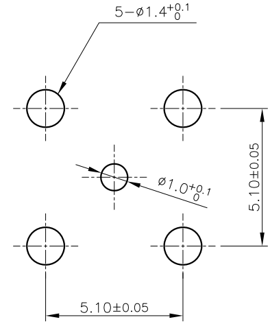
PCB MOUNTING HOLE
