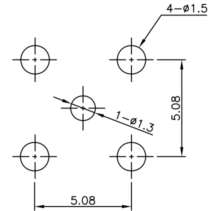
PCB MOUNTING HOLE SIZE
