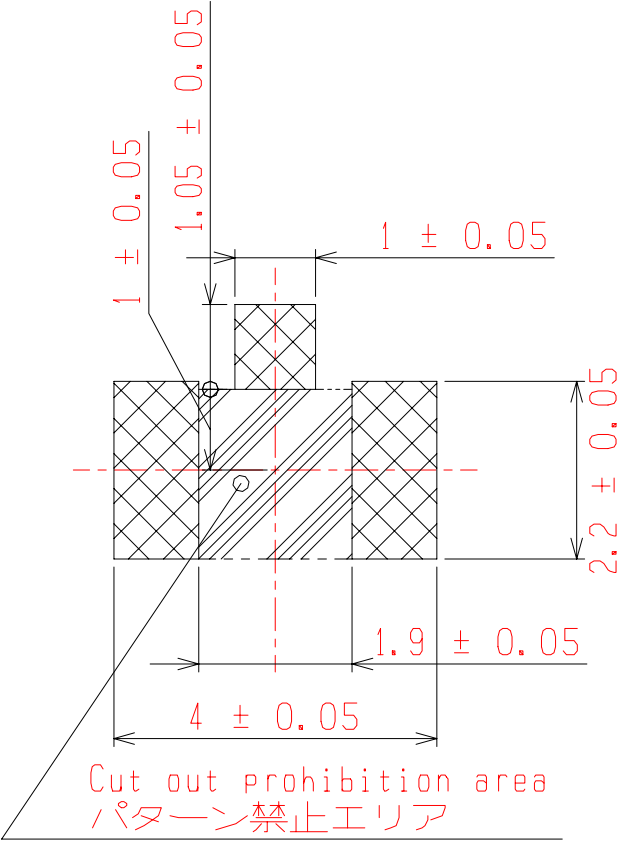
RECOMMENDED FOOTPRINT PATTERN
