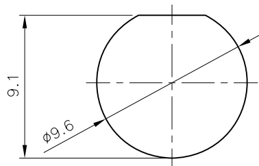
MOUNTING HOLE SIZE
