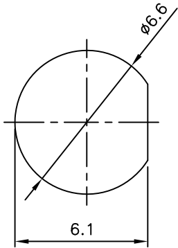
MOUNTING HOLE
