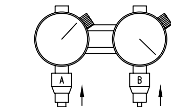
SMA FEMALE INTERFACE GAUGE - T6102
