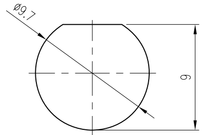
PANEL MOUNTING HOLE SIZE
