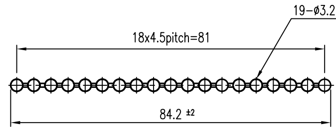
ROUND WIRE DETAIL
