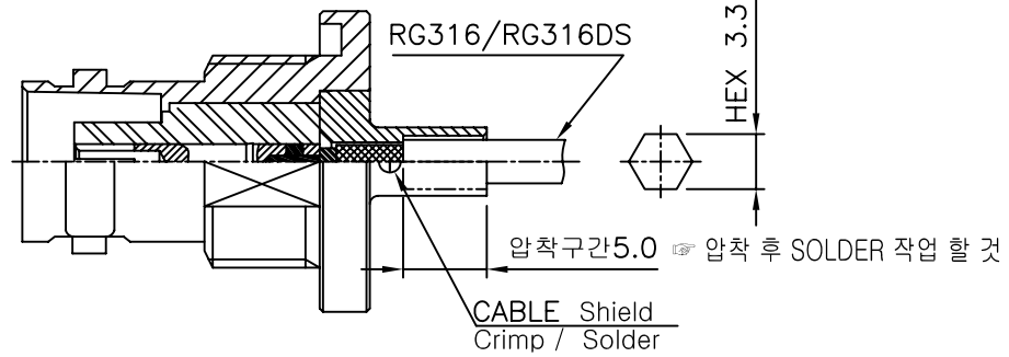
CABLE STRIPPING
