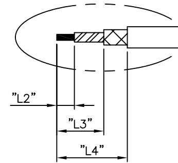
"A" Detail
