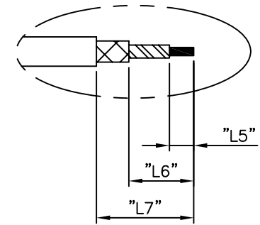
"B" Detail
