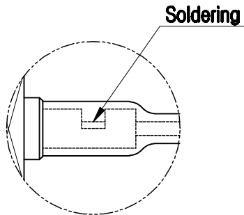
NO.2 CONNECTOR CABLE STRIPPING
