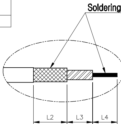
NO.2 CONNECTOR CABLE STRIPPING
