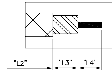
"A" Detail
