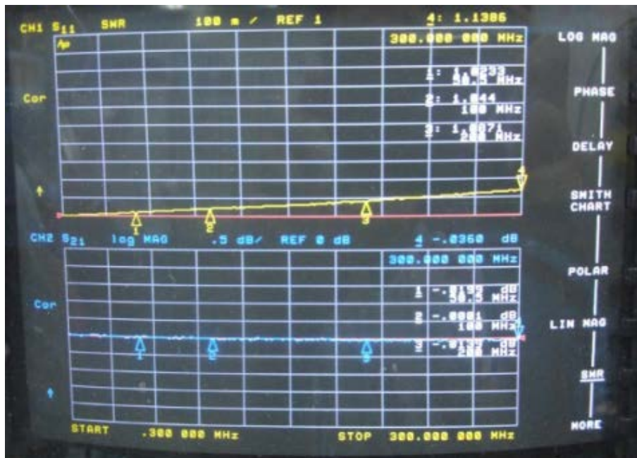
그림1) TR1 : IN Port VSWR, TR2: IN-OUT Insertion Loss
